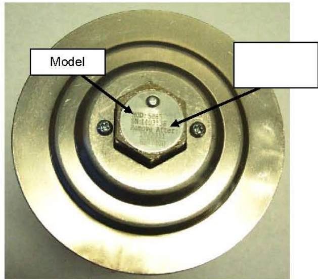
Husky 5885 P/V Vent Valve (Husky Name on Bottom Flange)
